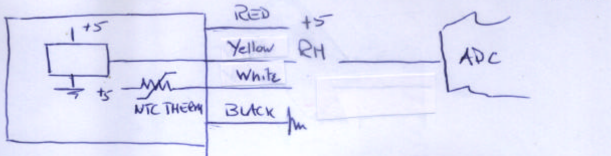
FIG #1 AHT11 UNIT
