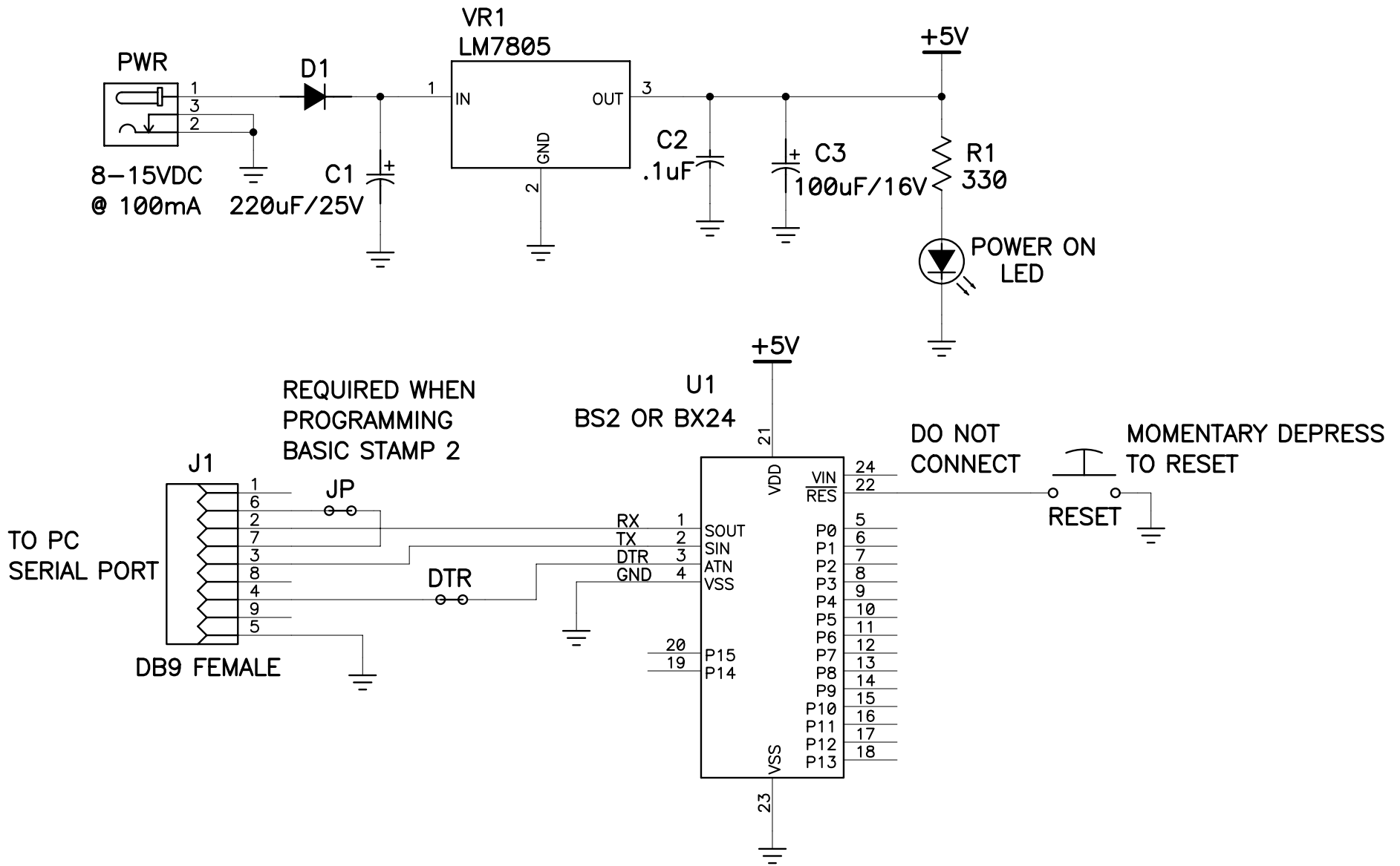
BS2 AND BX24 PROTO BOARD ANDERSON, FEB. '05
